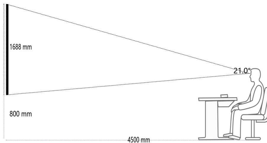
Figure 1.2.2 Vertical View
