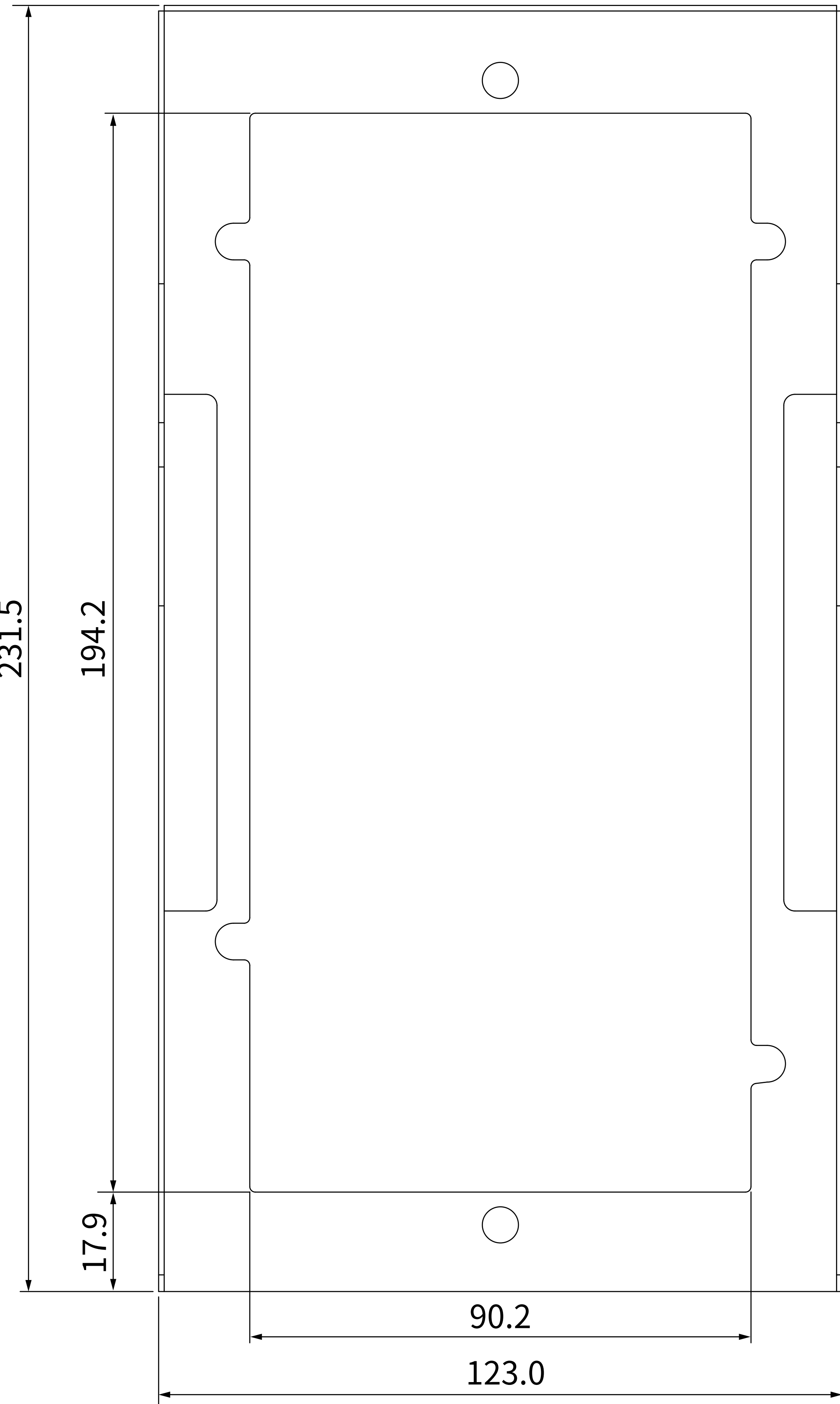
1 FRONT VIEW
