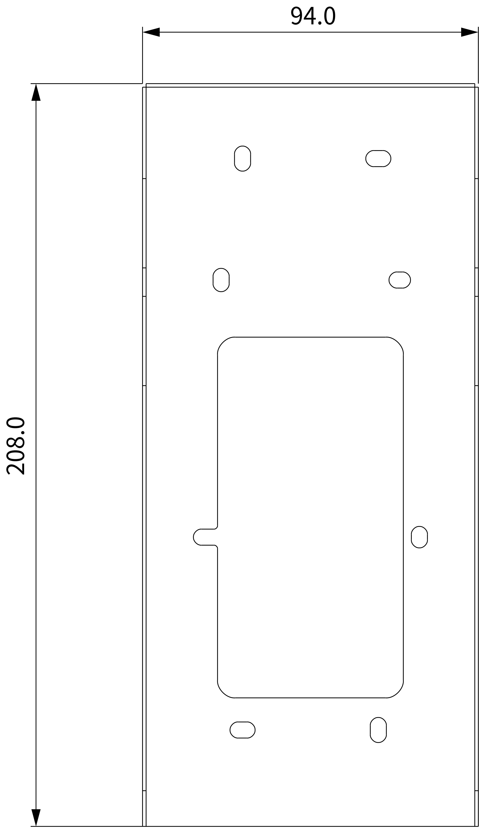
1 FRONT VIEW
