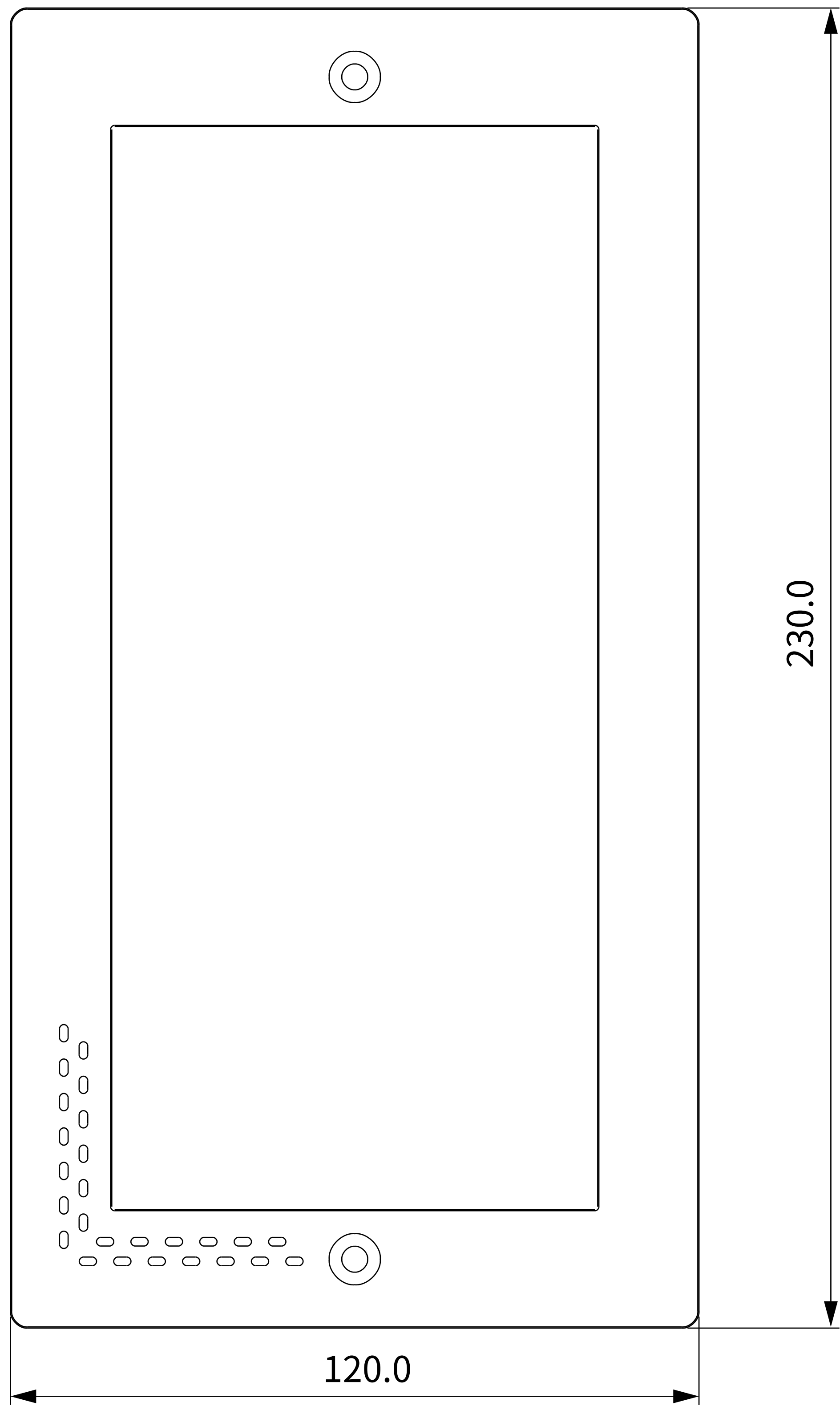
1 FRONT VIEW
