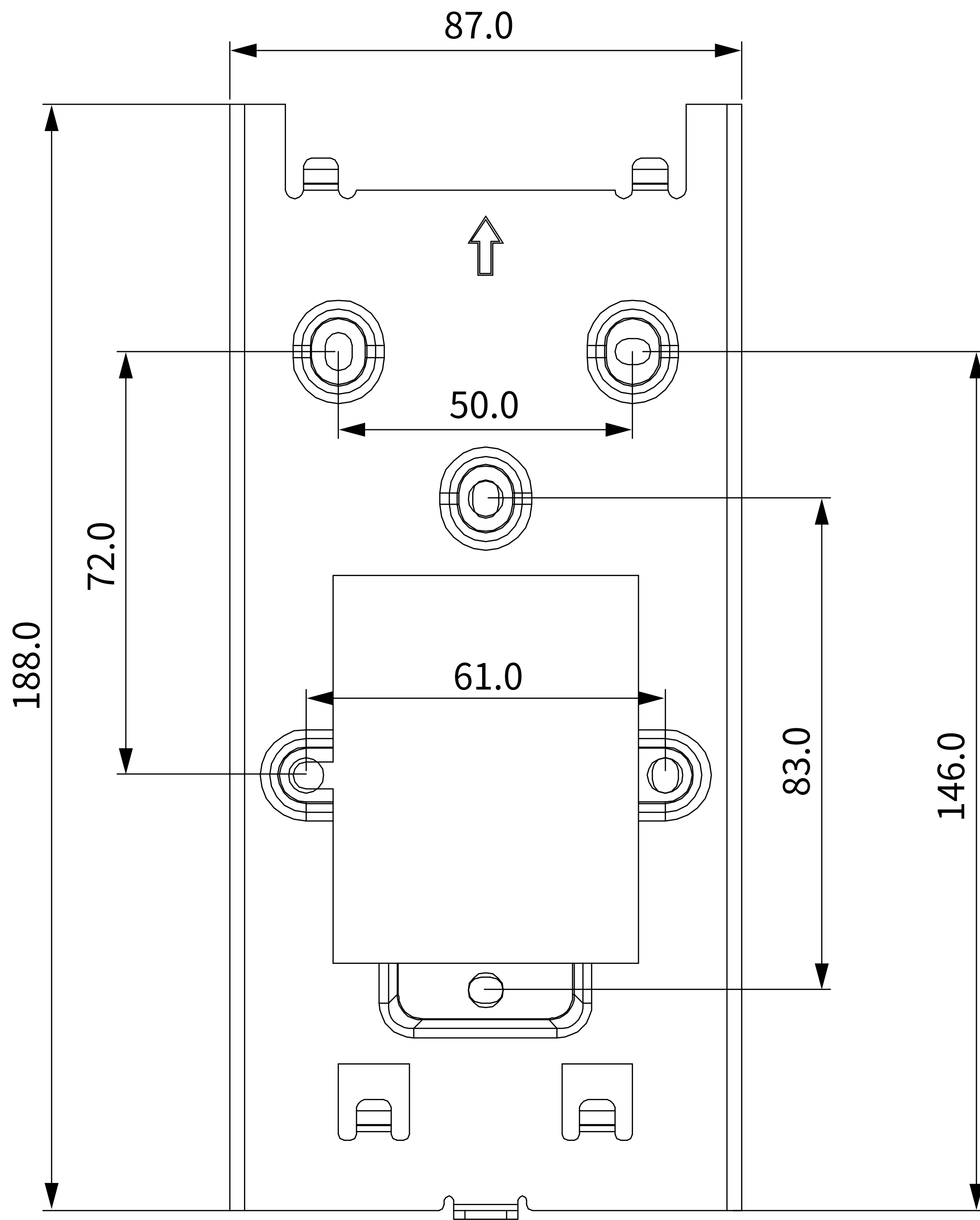
1 FRONT VIEW
