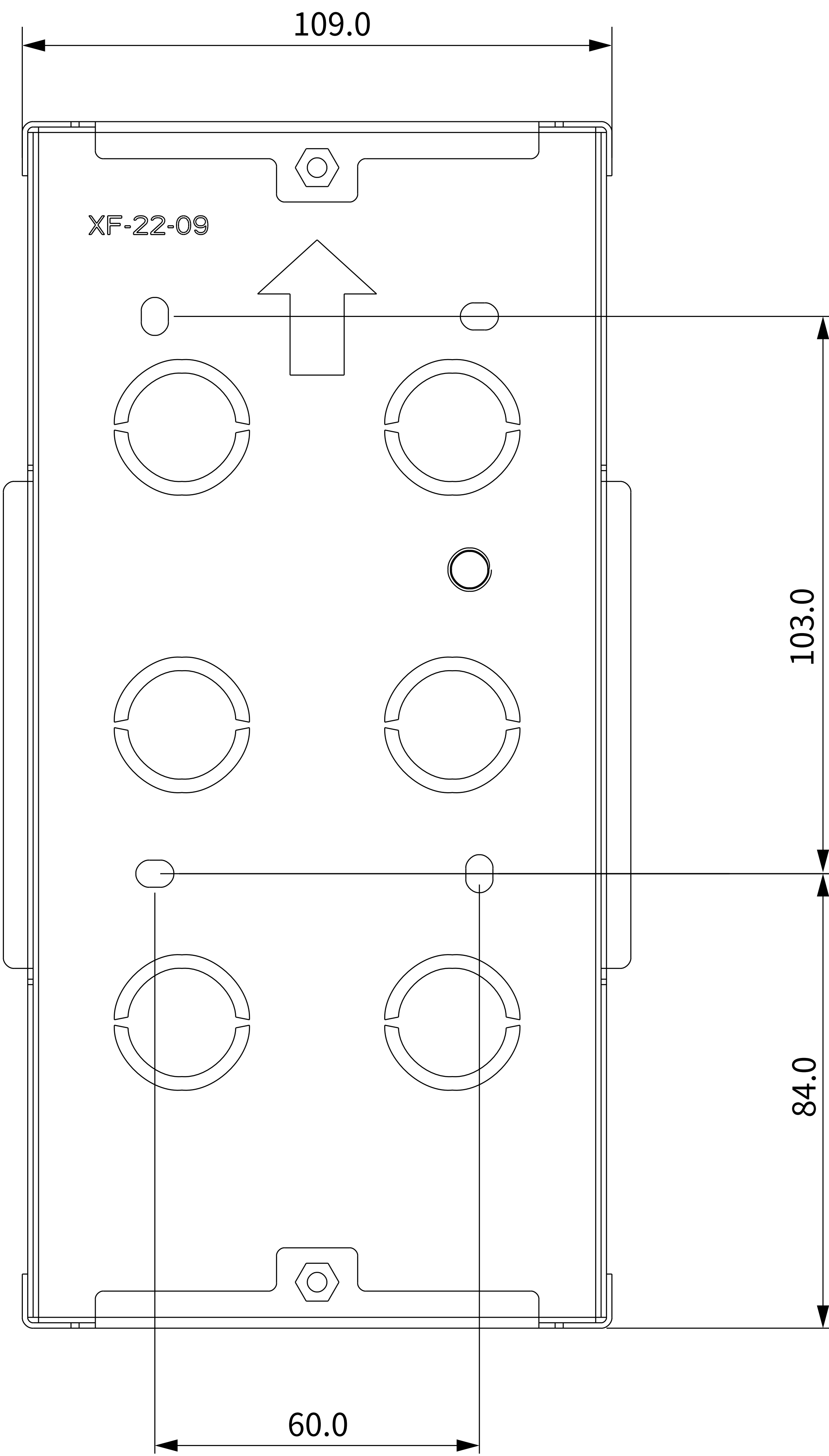
1 FRONT VIEW
