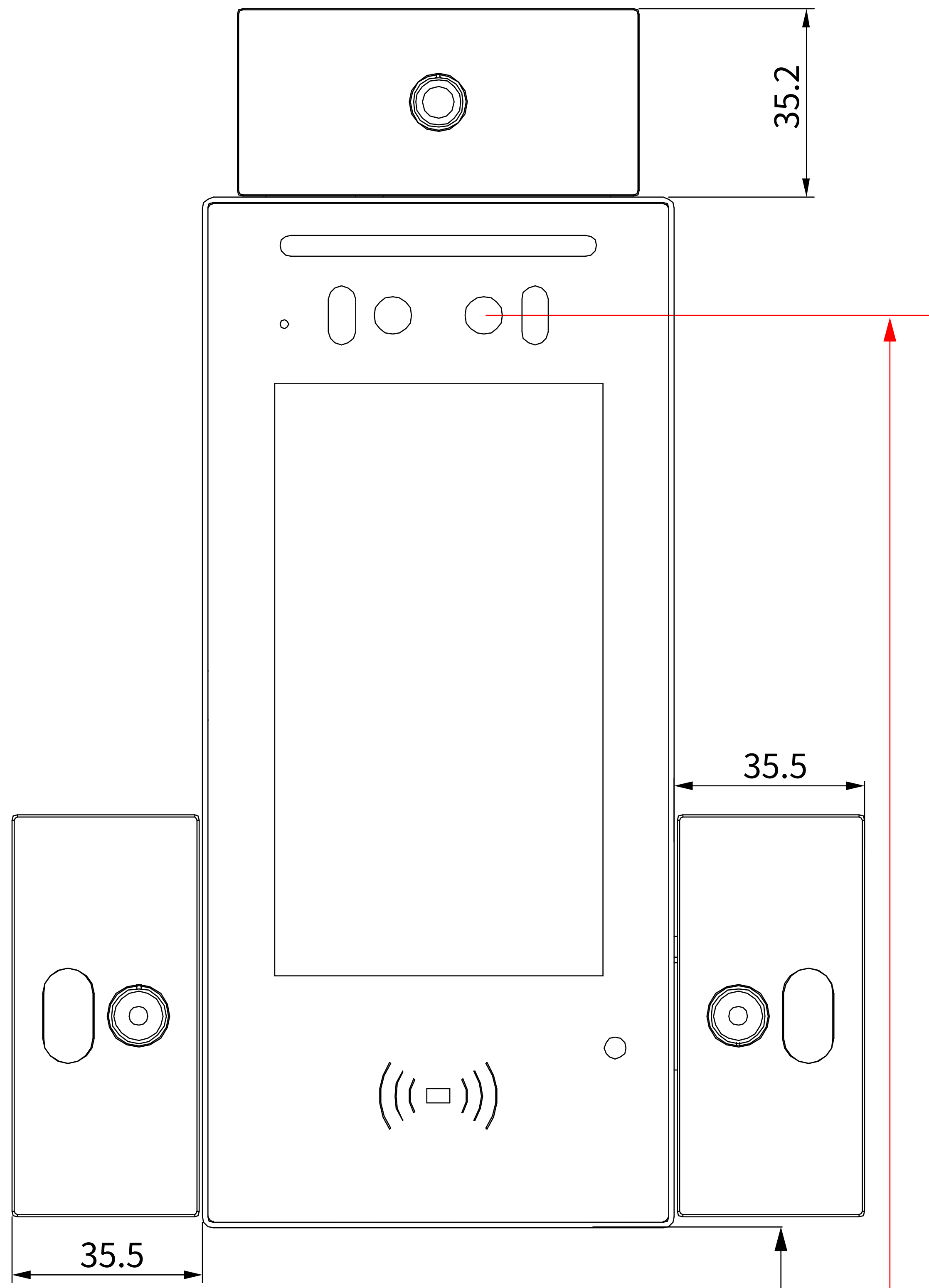
1 INTERCOM PANEL WITH TEMPERATURE MEASUREMENT MODULE FRONT VIEW
